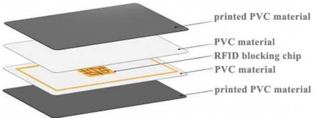
Structure RFID blocking card
